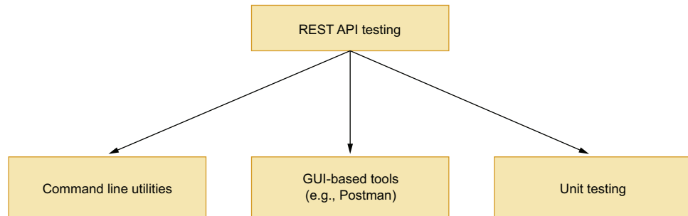
Figure 7.2 Options to test a RESTful API. Command line utilities includes cURL , HTTPie . The GUI-based tools include Postman , SoapUI . Unit testing can be done with Spring Boot MockMVC in conjunction with JUnit .
