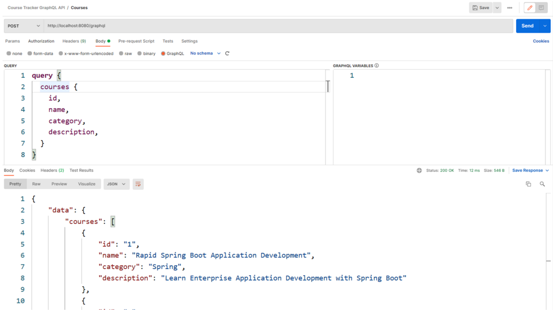
Figure 10.13 The GraphQL query request in Postman
