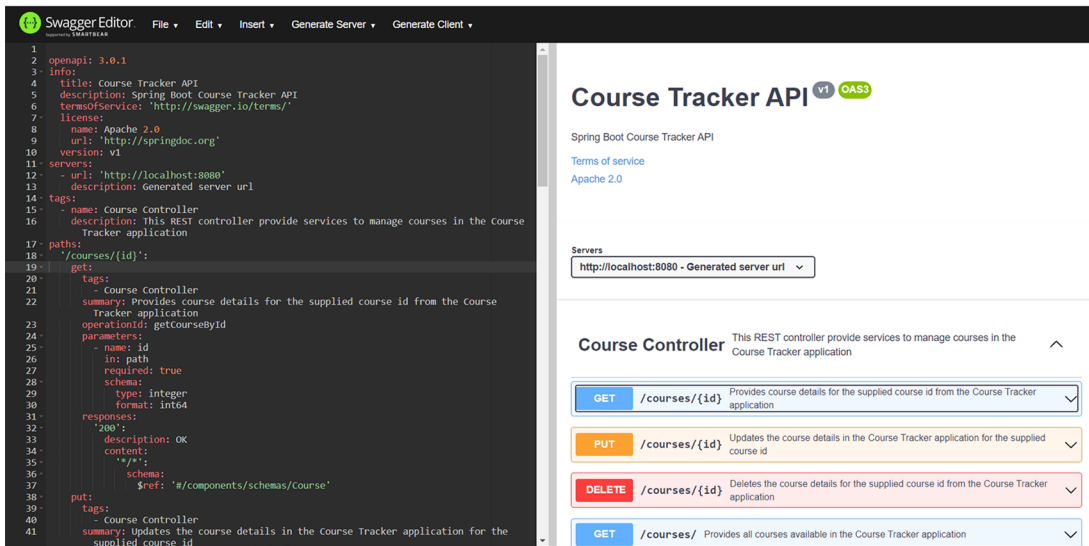
Figure 7.4 Rendering the REST API documentation in the Swagger Editor. The Swagger Editor prefers the YAML version of the JSON data and automatically converts a JSON to YAML while you paste the JSON in the editor.
