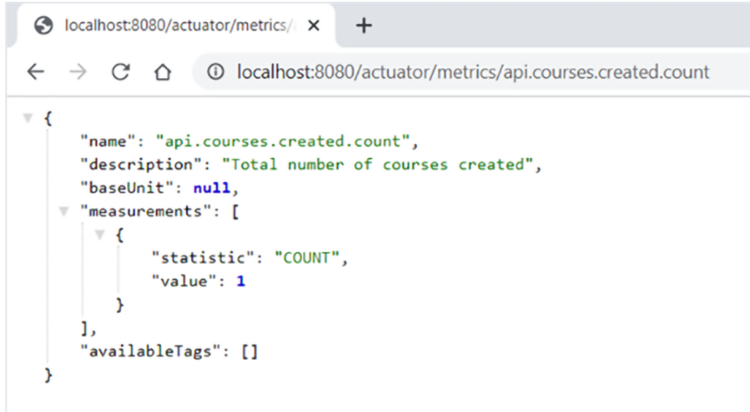
Figure 4.21 Outcome of the api.courses.created.count custom metric
